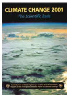
TAR 2001
