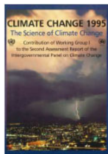
SAR 1995
